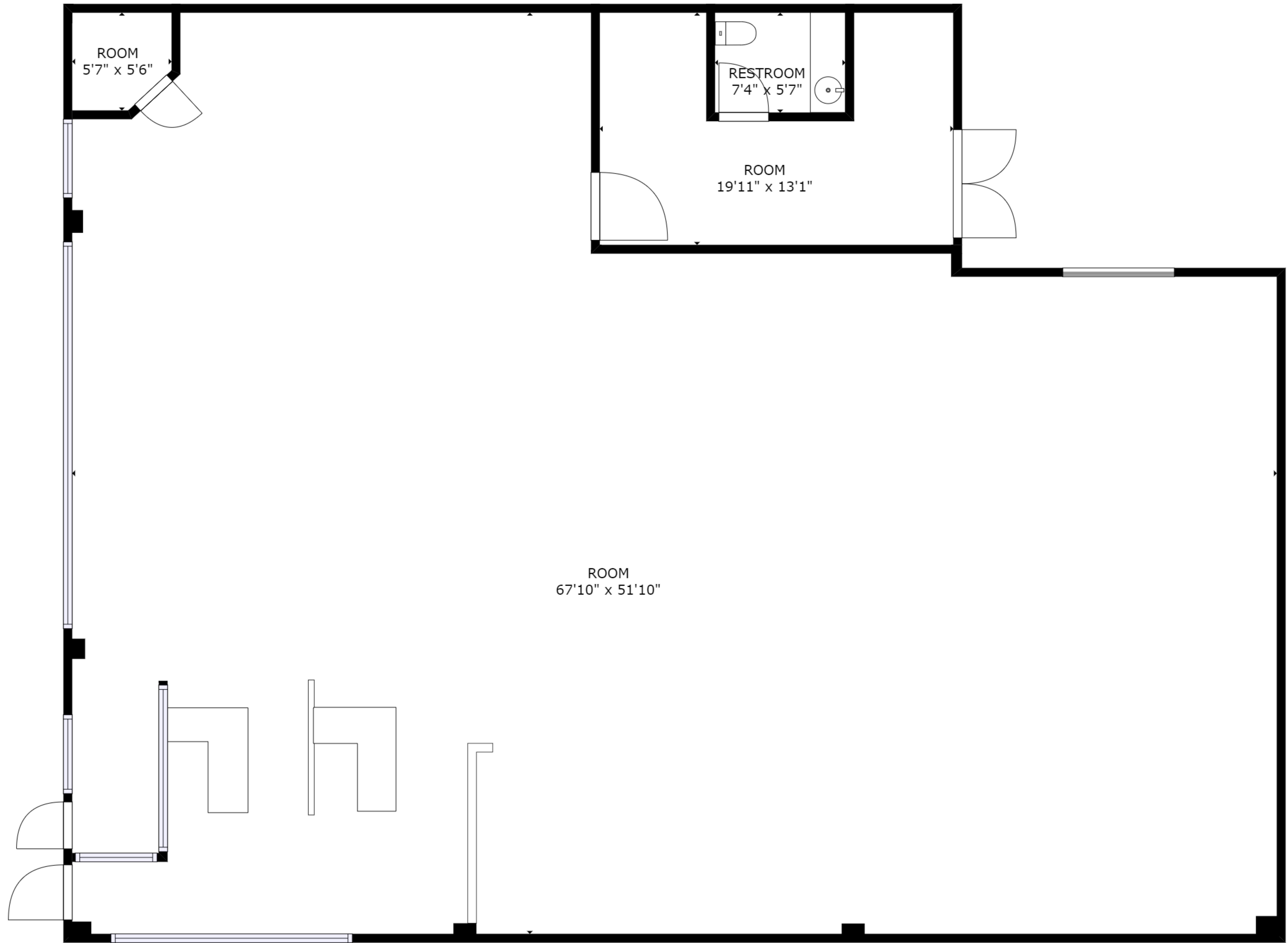
FLOOR 1
